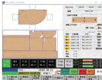
CNC Nesting
